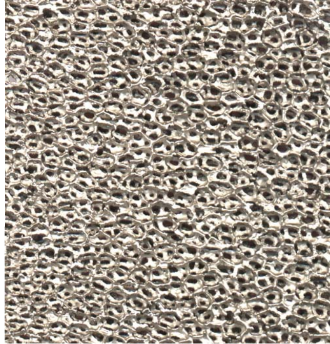
Photo: 1 Zirconia foam plated with LX for wear and abrasion protection.
